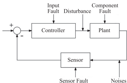
Fig. 2. Typical structure of an automatic control system and possible destructive factors
