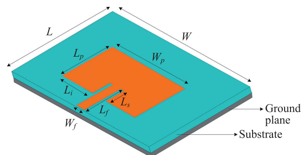
Fig. 1. Metamaterial-based MPA
